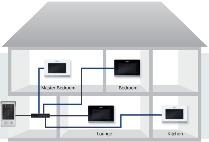
Single way IP system example components...
